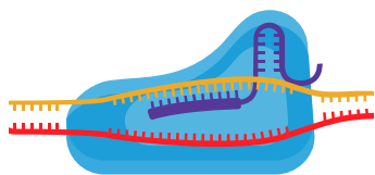
gRNA library construction for CRISPR
